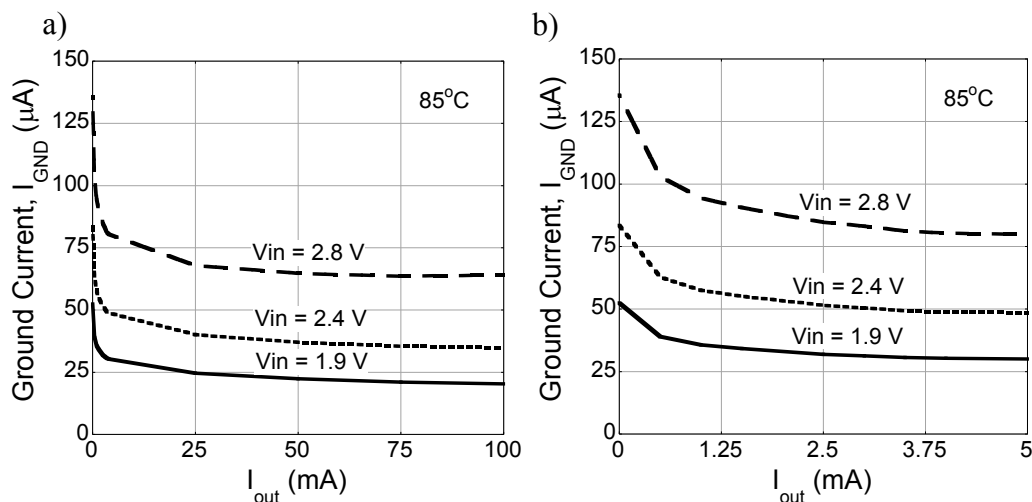
Fig. 76. a) Ground current at 85°C with the low I_q error amplifier. b) Ground current at 85°C with the low I_q error amplifier at light loads.
