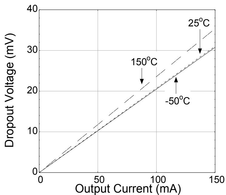
Fig. 75. The dropout voltage was measured up to 100 mA for -50, 25, and +150°C and extrapolated from 100 to 150 mA.
