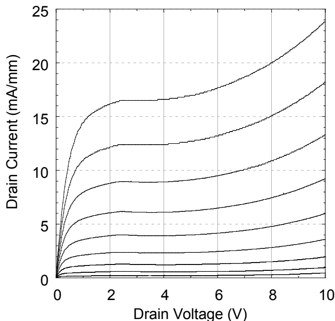
Fig. 25. The family of curves for a MESFET with L_g = 400 nm, L_{aS} = 600 nm and L_{aD} = 1 \mu m. The gate voltage is stepped from +0.4 V (uppermost curve) to -0.4 V in 0.1 V steps.
