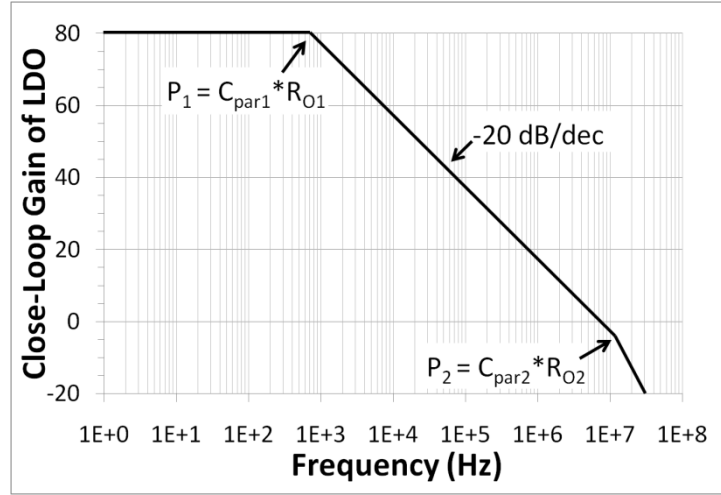
Fig. 52. Closed-loop gain response of an LDO utilizing a NMOS pass transistor.
