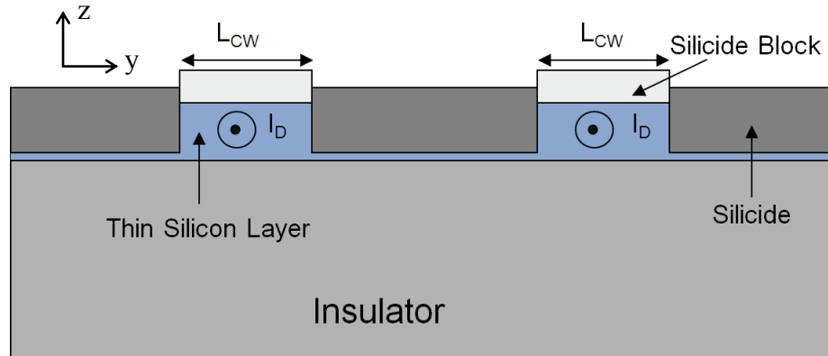
Fig. 28. Shows a cross-section in the y-z plane through the center of the device. The conducting channels are formed underneath the regions of silicide block. The current flows into the channels as indicated in the figure [27].
