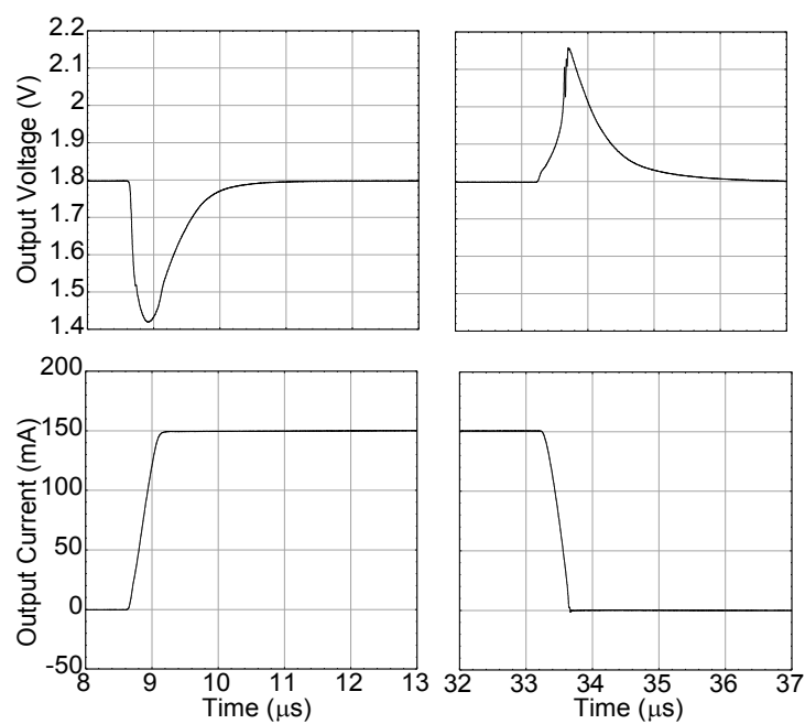
Fig. 96. Transient load regulation with the moderate I_q error amplifier after 1 Mrad(Si). V_{in} = 2.4 V, t_r = t_f = 500 ns and T = 50 μs.
