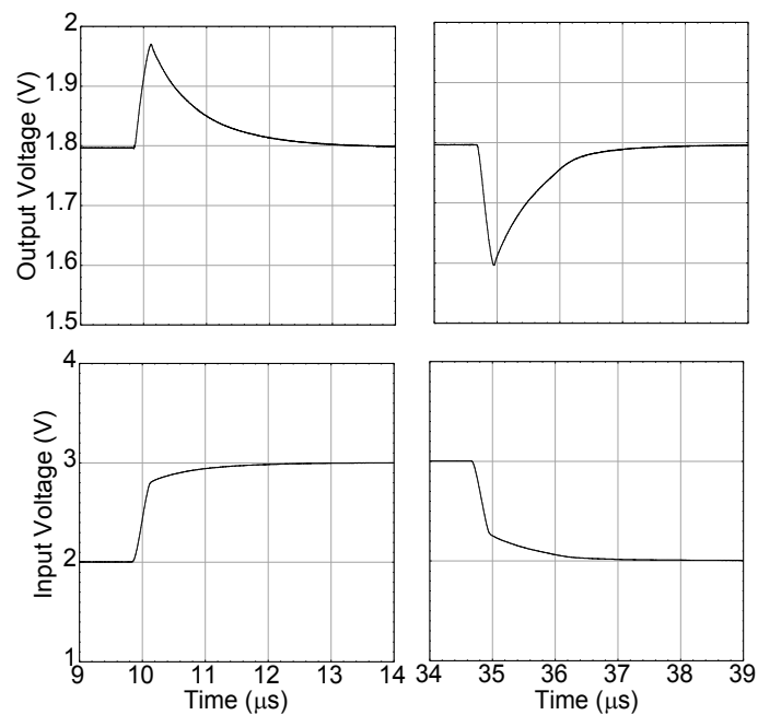
Fig. 95. Transient line regulation with the moderate I_q error amplifier after 1 Mrad(Si). I_{out} = 50 mA, t_r = t_f = 200 ns and T = 50 μs.
