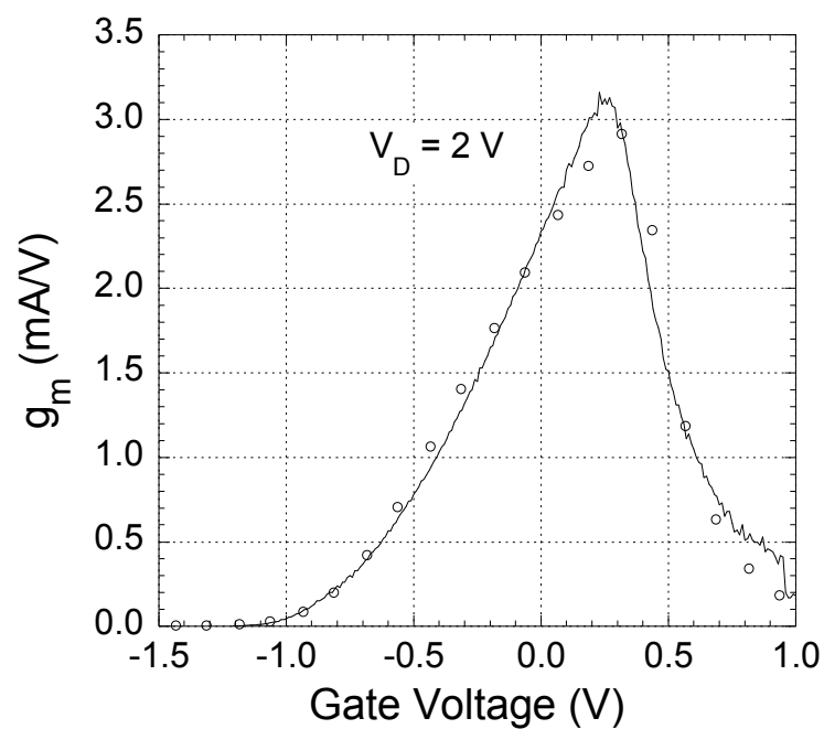
Fig. 45. Compares the g_m of the measured results (solid line) to the simulated model (open circles) at V_D = 2\text{ V} .
