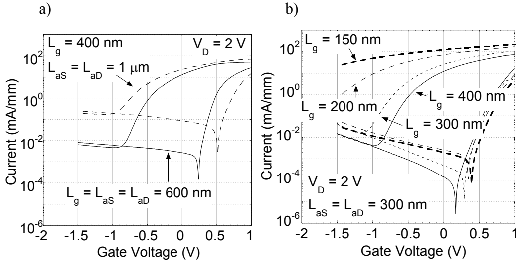
Fig. 15. Gummel plots for the smallest gate lengths fabricated on each process: a) 350 nm SOI CMOS and b) 150 nm SOI CMOS.
