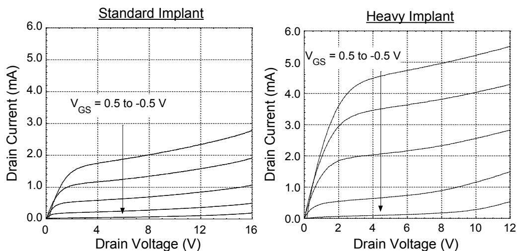
Fig. 35. Compares the FOC for two devices that are nominally the same but with different doping profiles. The heavier doping improved the current drive and output resistance, but reduced the breakdown voltage of the device.
