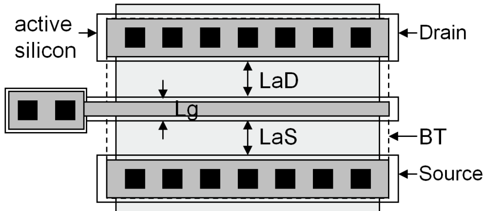
Fig. 13. Top-view of the BT PD-MESFET layout with the gate contacted outside the access region to reduce L_g .
