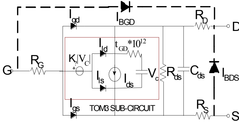
Fig. 41. Large signal model of a MESFET with the TOM3 sub-circuit. I_{BGD} and I_{BDS} are used to model the breakdown voltage in the circuit [23].
