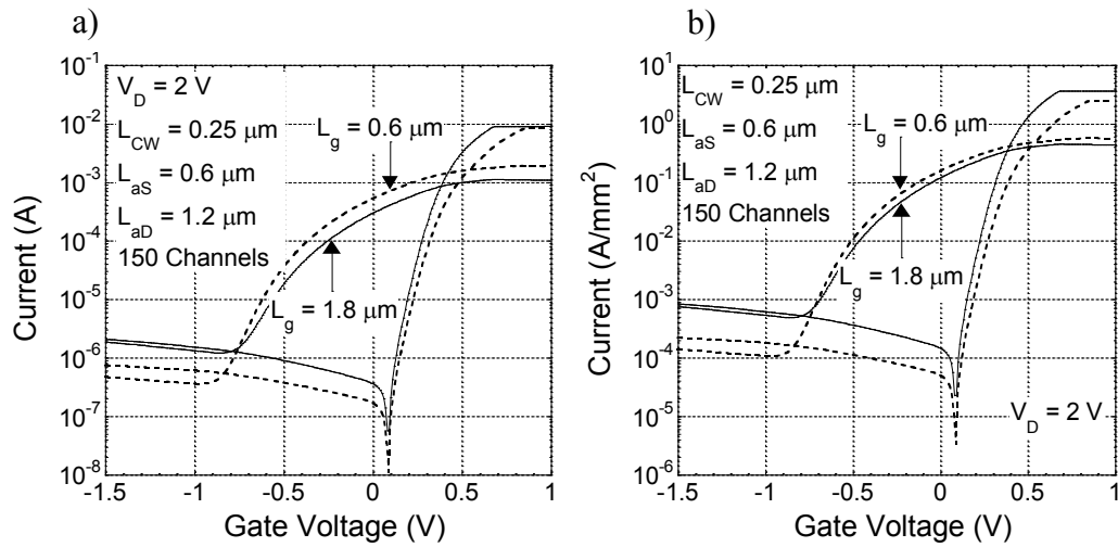
Fig. 37. a) Compares two devices, that are nominally similar except one utilizes the structure in Fig. 27 ( L_g = 1.8 \text{ } \mu\text{m} --solid line) and the other uses Fig. 36 ( L_g = 0.6 \text{ } \mu\text{m} --dashed line). b) Compares the two devices after they have been normalized to current per unit area.
