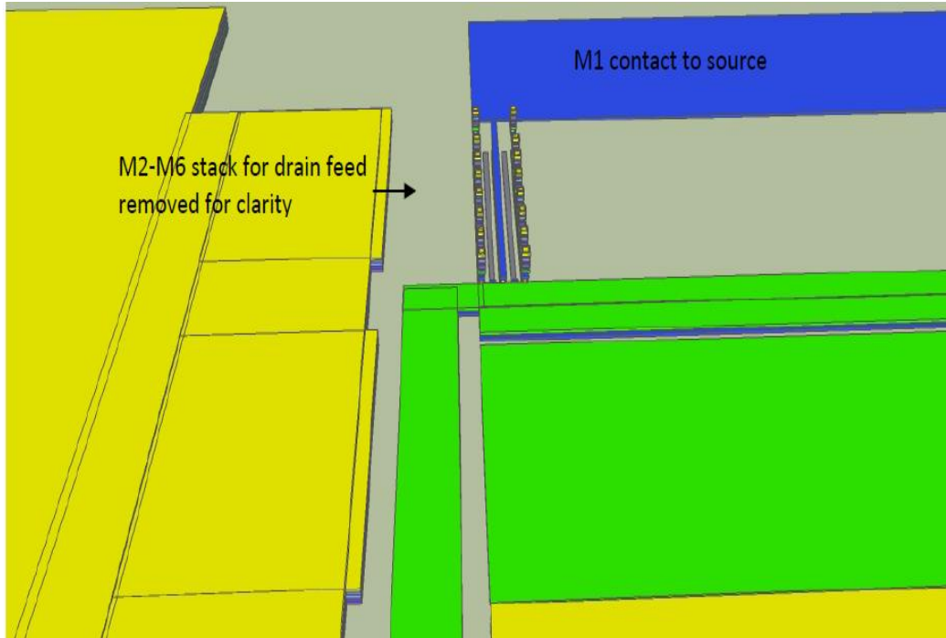
Fig. 103. Removes the entire drain line and some of the metal layers of the source and gate lines in Fig. 102 to show how individual fingers connect to the bus lines. All but two of the fingers were removed to simplify the picture.
