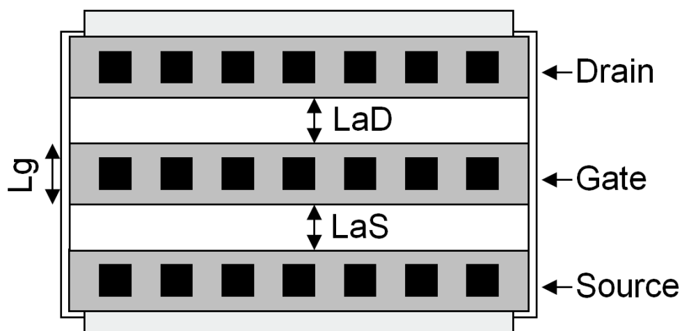
Fig. 11. Top-view of PD-MESFET layout with the gate contacted inside the access region (silicide block is used to create the \text{SiO}_2 spacers).
