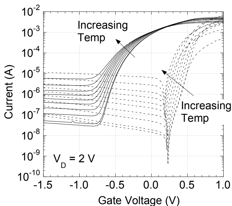
Fig. 7. The Gummel plot shows the changes in DC operation for a 100\text{ }\mu\text{m} device with L_g = L_{aS} = L_{aD} = 0.6\text{ }\mu\text{m} between -60 to 150\text{ }^\circ\text{C} . From -50 to 150\text{ }^\circ\text{C} the temperature steps in 25\text{ }^\circ\text{C} increments. The solid lines are I_D while the dotted lines are the magnitude of I_G . The device is from a 350\text{ nm} SOI CMOS process.
