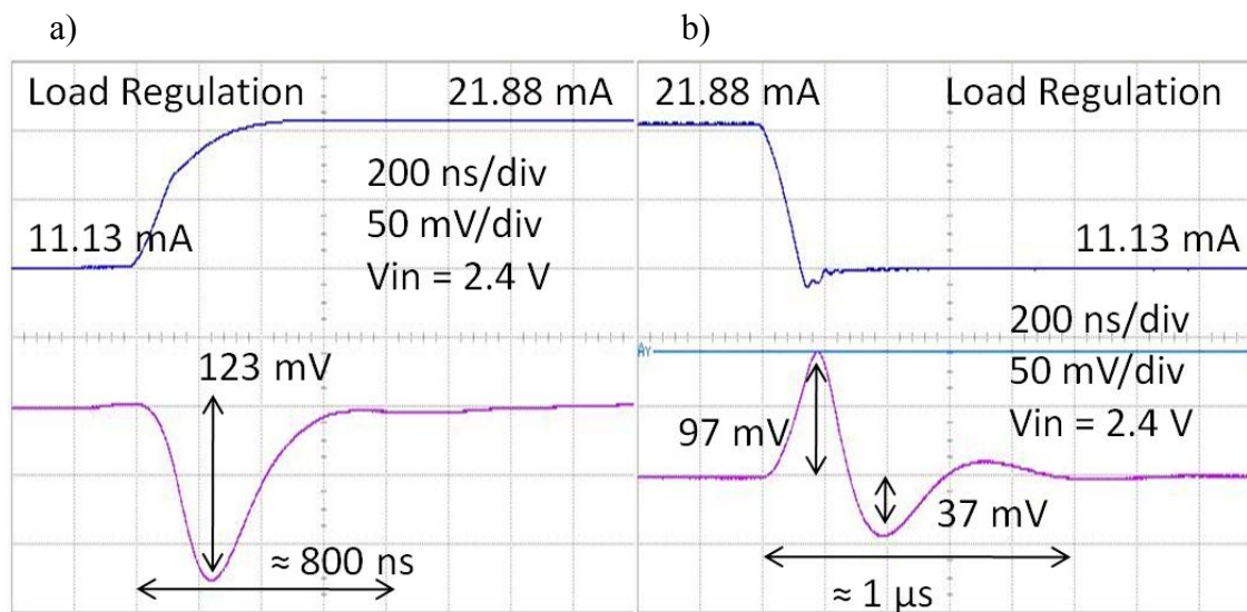
Fig. 60. Measured load regulation for both the low-to-high, a), and high-to-low transitions, b). The output voltage settles in less than \leq 1 \mu s.
