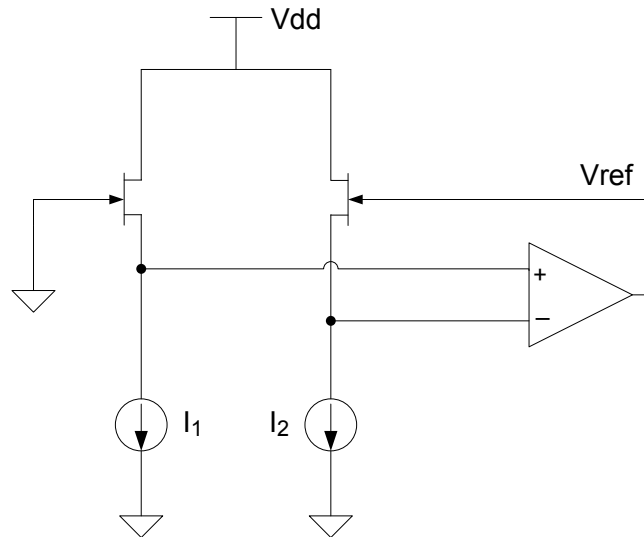
Fig. 8. Structure of the MESFET PTAT used in [12].
