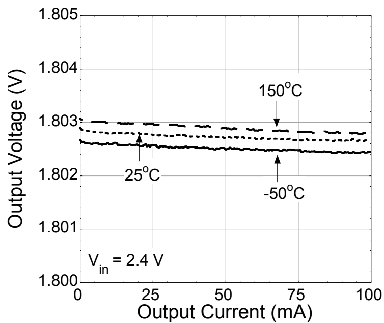
Fig. 74. Load regulation at -50, 25, and +150°C at a V_{in} = 2.4\text{ V} .
